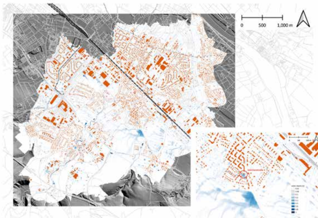
Figure 1: Simulated maximum surface inundation for the heavy precipitation event of 27th May, 2014 in the Lockwitzbach area of Dresden. The inset shows a plausibility check, comparing a reported basement inundation of a building (red circle) with the simulated inundation.
