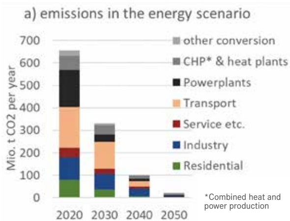
Figure 1: Necessary reduction in CO 2 emissions from the energy system to limit climate change below 2°C (Simon et al., 2022)
