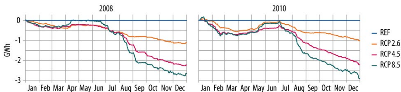
Figure 3. Cumulated deviations of the electricity generation from the selected onshore wind turbines for three different climate scenarios compared to the reference values of the years 2008 and 2010.
