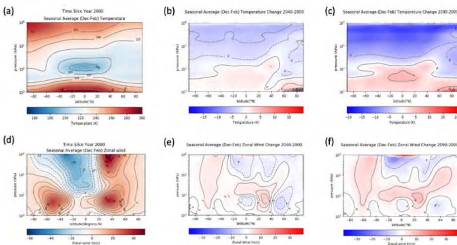
Fig. 2 Zonal-mean and seasonal-mean (DJF) (a) temperature as a function of latitude and pressure, (b)–(c) difference in temperature for the years 2040–2000 and 2090–2000, (d) corresponding zonal wind, and (e)–(f) difference in zonal wind for the years 2040–2000 and 2090–2000.
